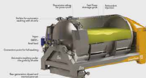
Smart Press closed cage SPD 110 - cutaway view
